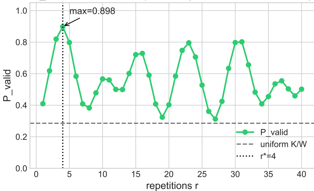
P_valid oscillation vs repetitions (theta=0.524, beta=0.300)
