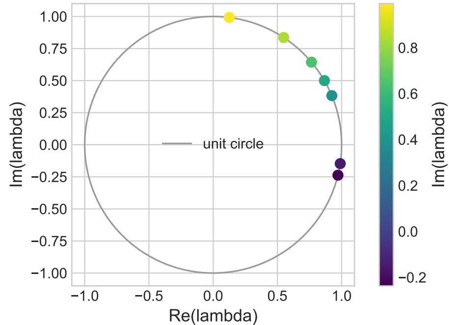
Eigenvalue spectrum of one layer — V4
