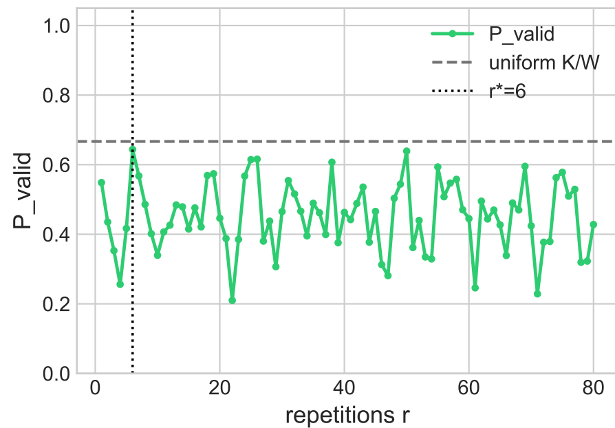
Oscillation
