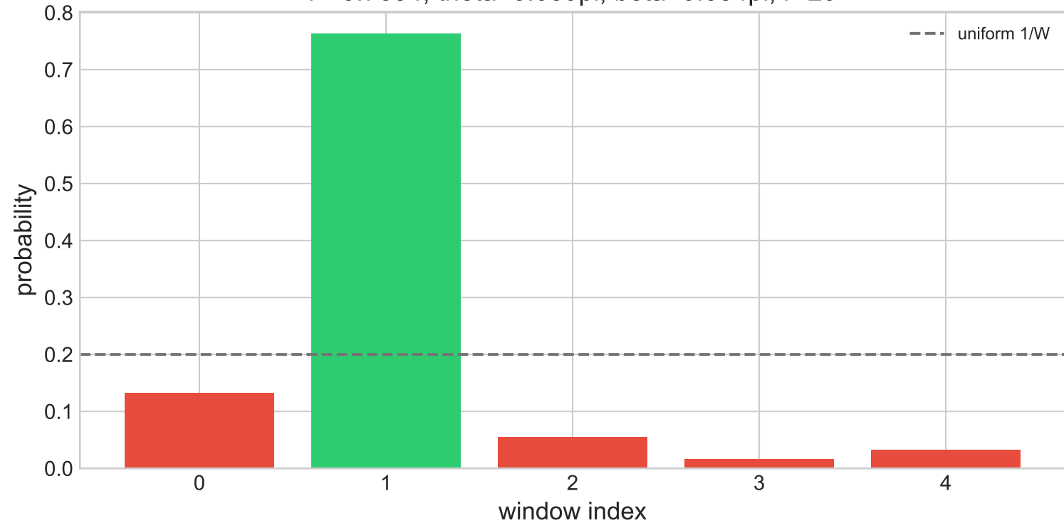
Optimal distribution - 01_1d_tiny_single_gap P=0.7634 , \theta=0.089\pi , \beta=0.054\pi , r=29
