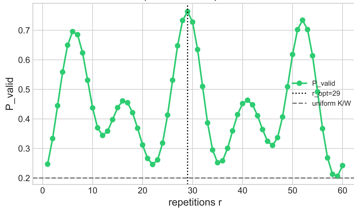
Oscillation - 01_1d_tiny_single_gap \theta=0.089\pi , \beta=0.054\pi , r=29 , P=0.7634
