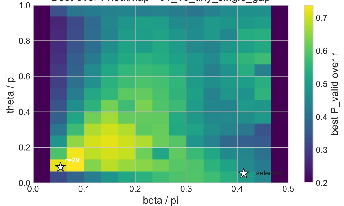
Optimal distribution - 01_1d_tiny_single_gap P=0.7634 , \theta=0.089\pi , \beta=0.054\pi , r=29
