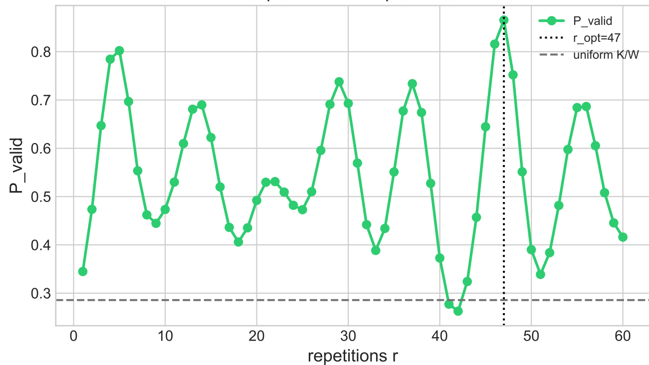
Oscillation - 04_1d_clustered_medium \theta=0.107\pi , \beta=0.107\pi , r=47 , P=0.8655
