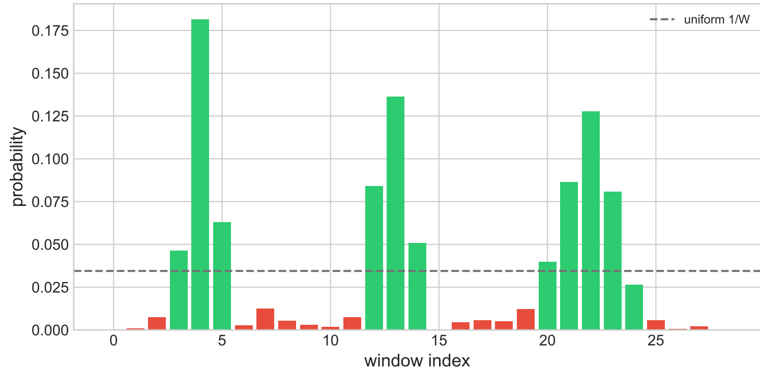
Optimal distribution - 05_1d_long_clustered_blocks P=0.9229 , \theta=0.018\pi , \beta=0.040\pi , r=23
