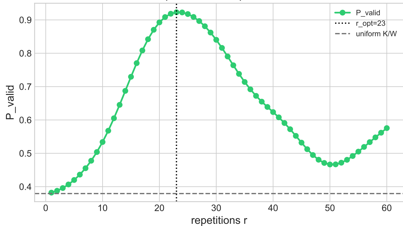
Oscillation - 05_1d_long_clustered_blocks \theta=0.018\pi , \beta=0.040\pi , r=23 , P=0.9229
