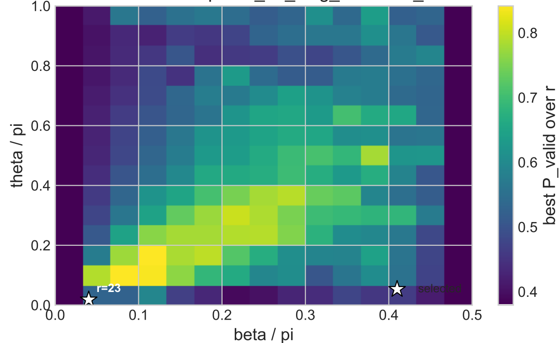
Optimal distribution - 05_1d_long_clustered_blocks P=0.9229, theta=0.018pi, beta=0.040pi, r=23
