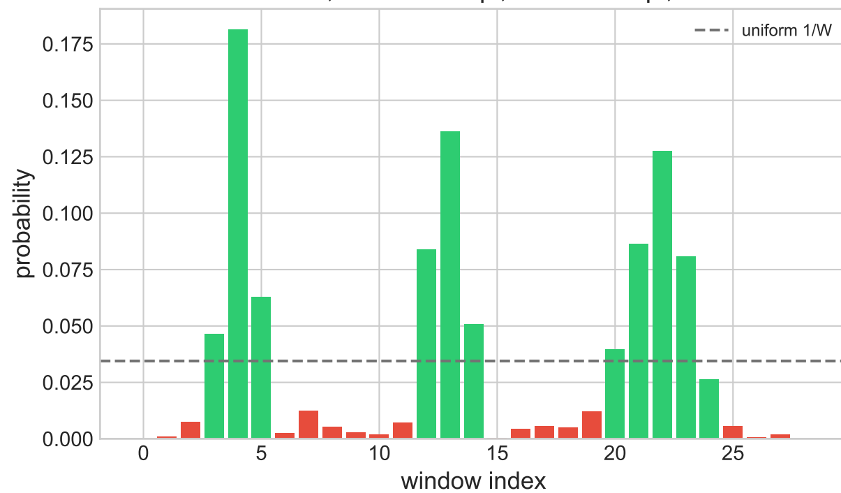
Optimal distribution - 05_1d_long_clustered_blocks P=0.9229, theta=0.018pi, beta=0.040pi, r=23
