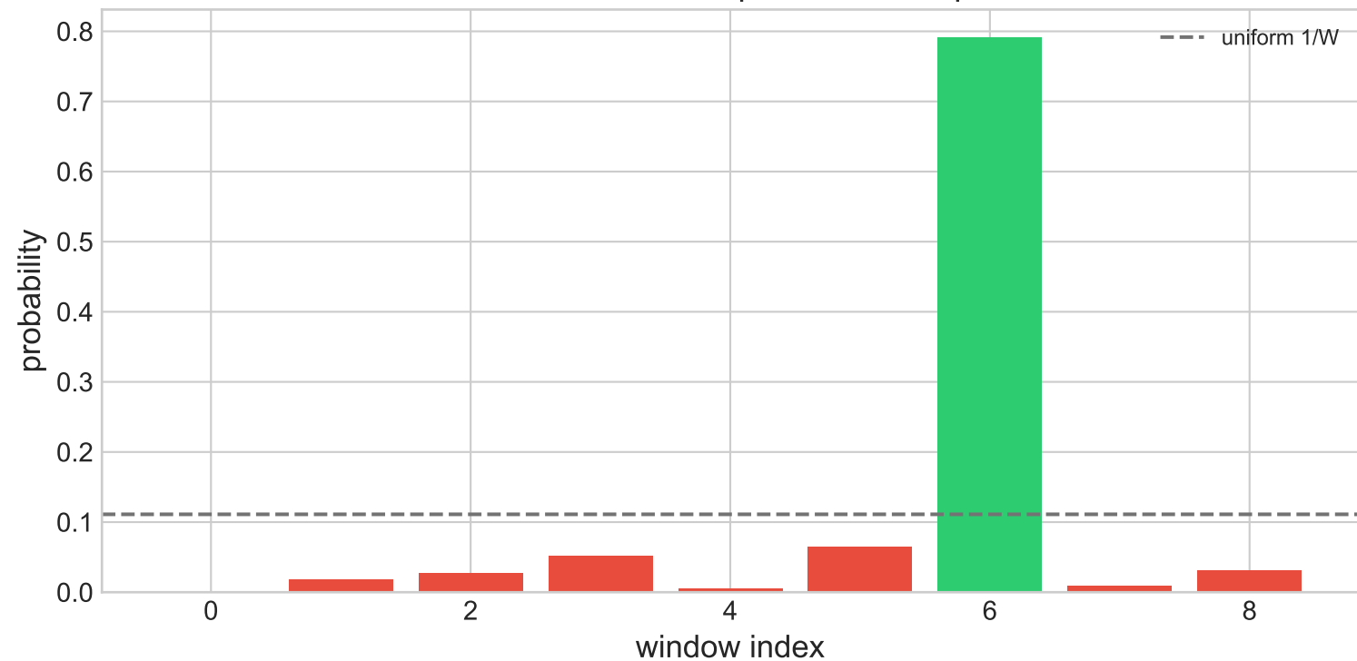
Optimal distribution - 07_2d_small_diagonal_block P=0.7915 , \theta=0.125\pi , \beta=0.054\pi , r=48
