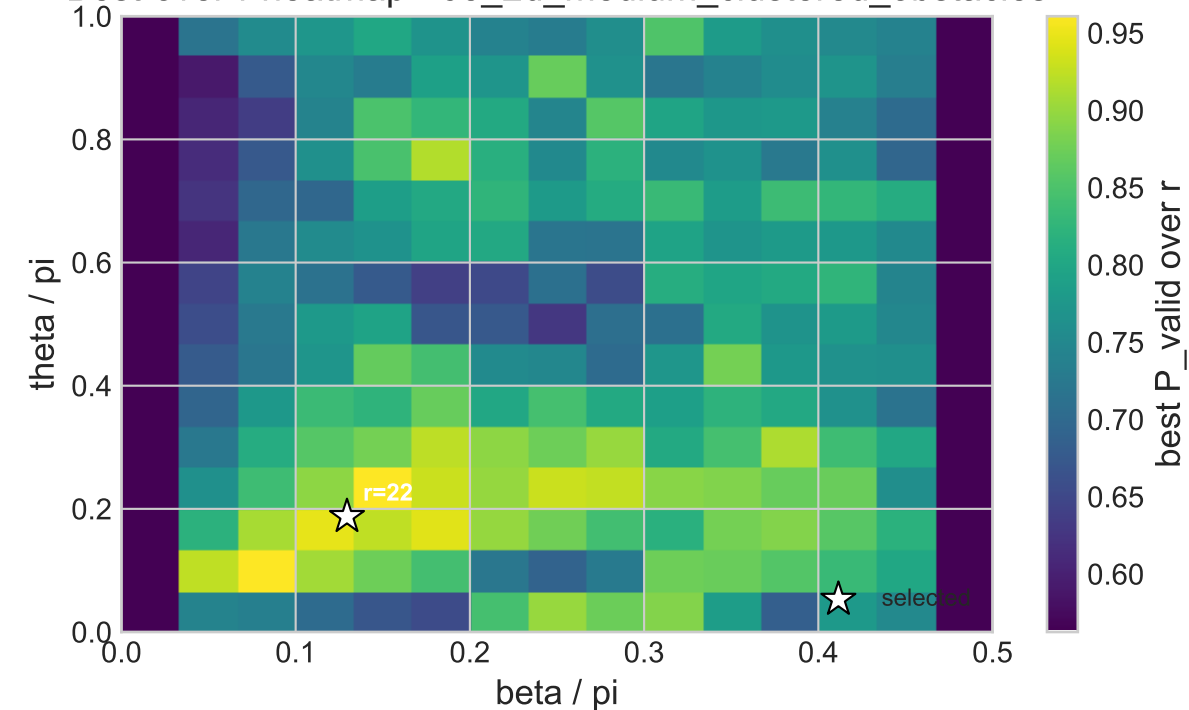
Optimal distribution - 08_2d_medium_clustered_obstacles P=0.9831, theta=0.188pi, beta=0.129pi, r=22
