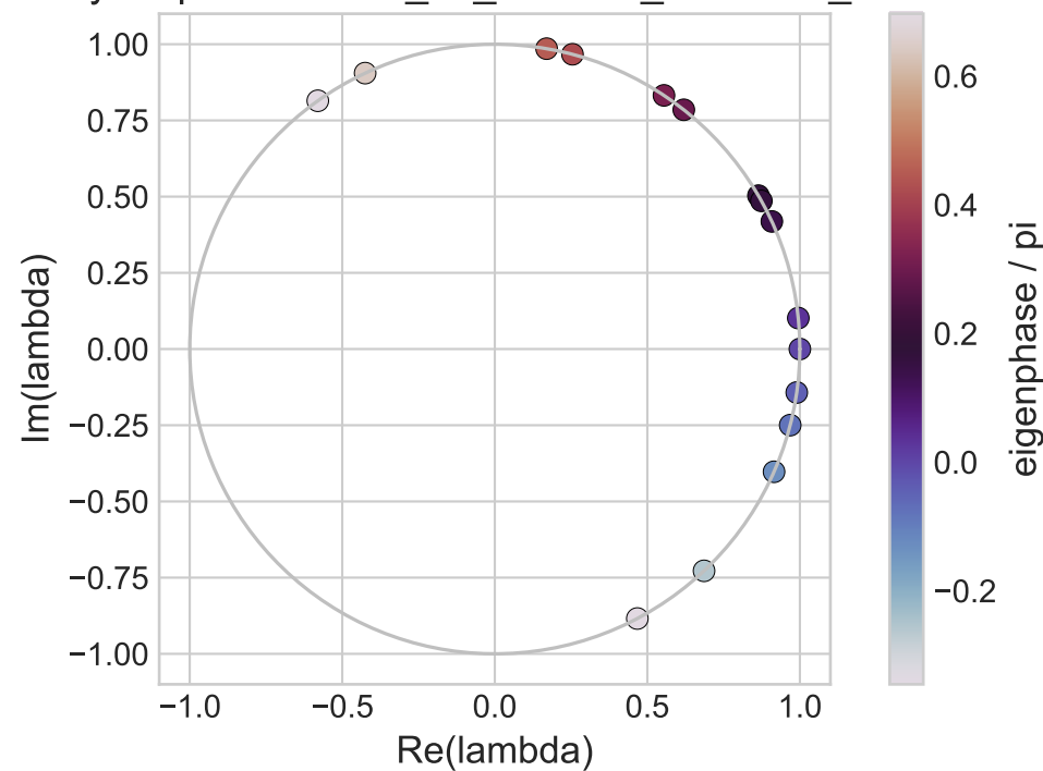
One-layer spectrum - 08_2d_medium_clustered_obstacles
