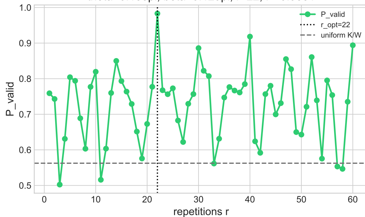
Oscillation - 08_2d_medium_clustered_obstacles theta=0.188pi, beta=0.129pi, r=22, P=0.9831
