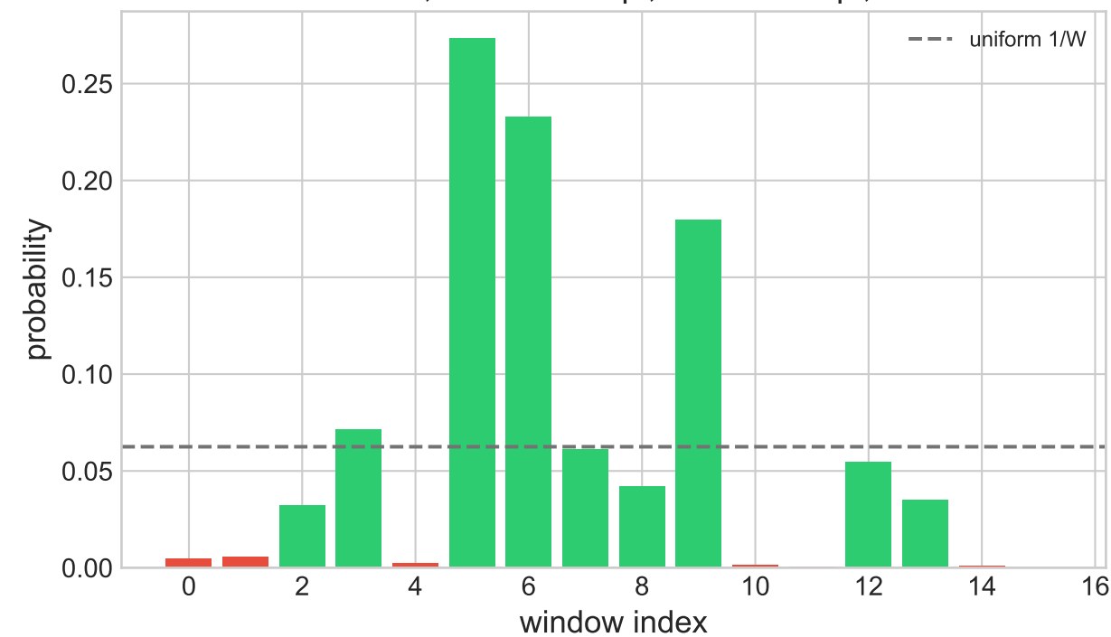
Optimal distribution - 08_2d_medium_clustered_obstacles P=0.9831, theta=0.188pi, beta=0.129pi, r=22
