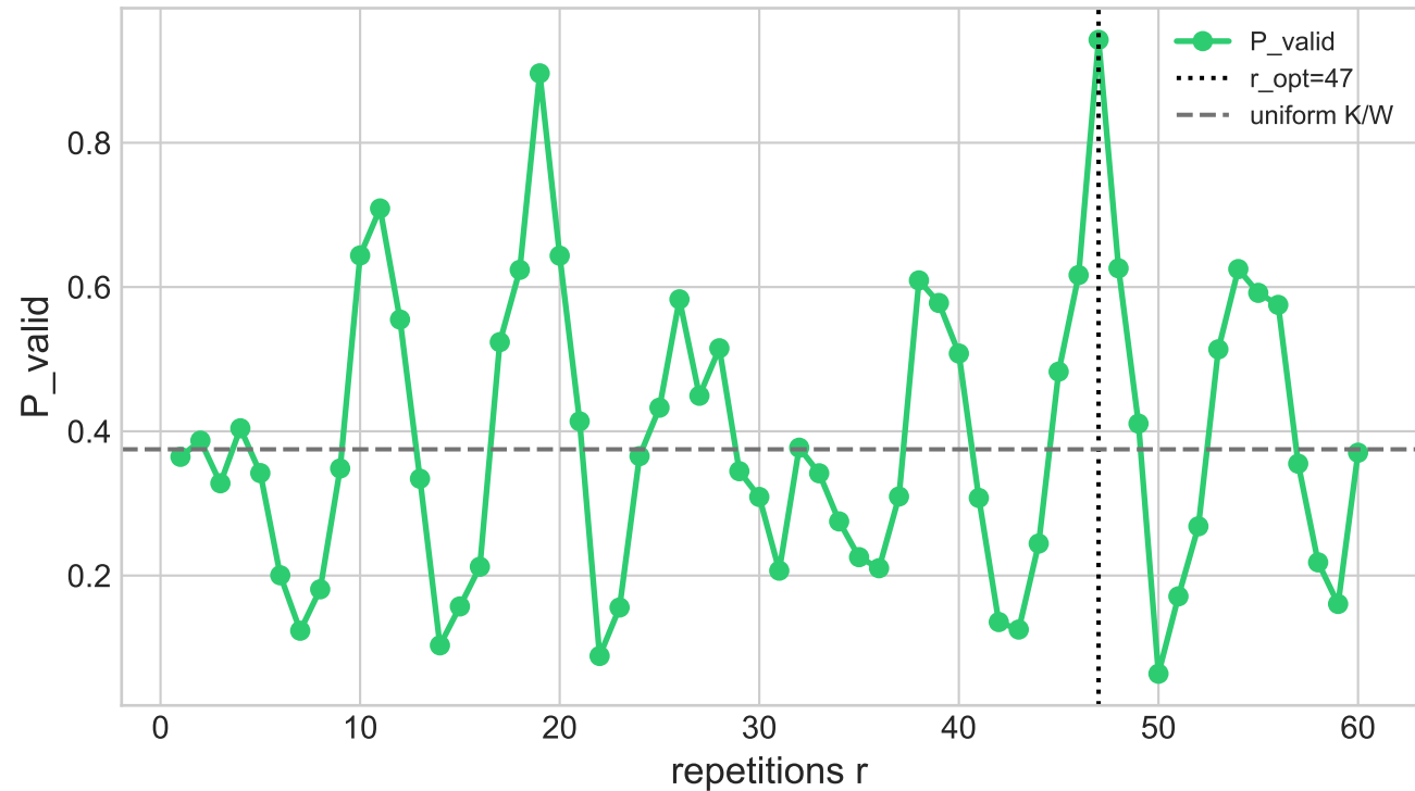
Oscillation - 03_1d_two_free_regions \theta=0.152\pi , \beta=0.344\pi , r=47 , P=0.9427
