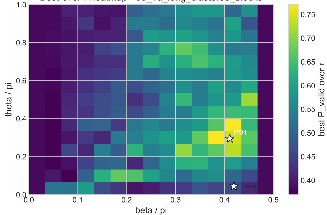
Best-over-r heatmap - 05_1d_long_clustered_blocks
