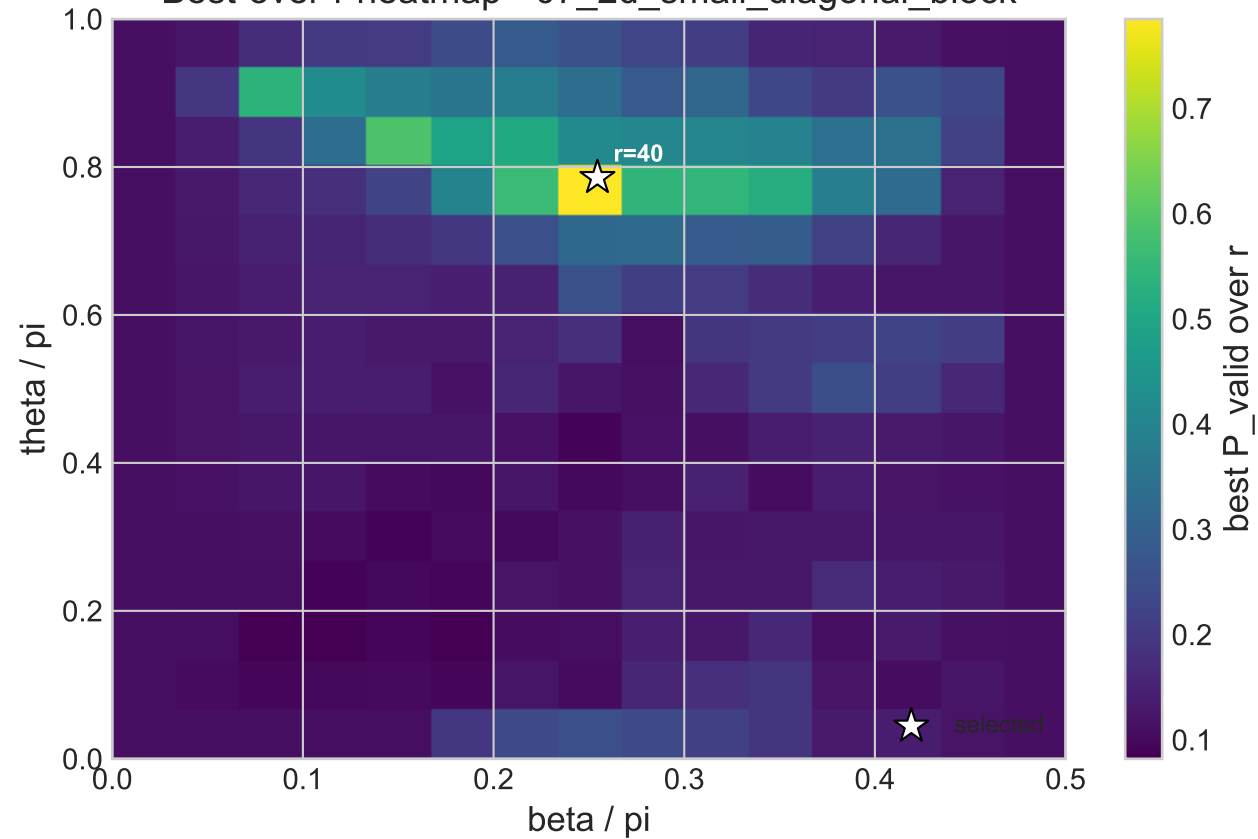
Best-over-r heatmap - 07_2d_small_diagonal_block
