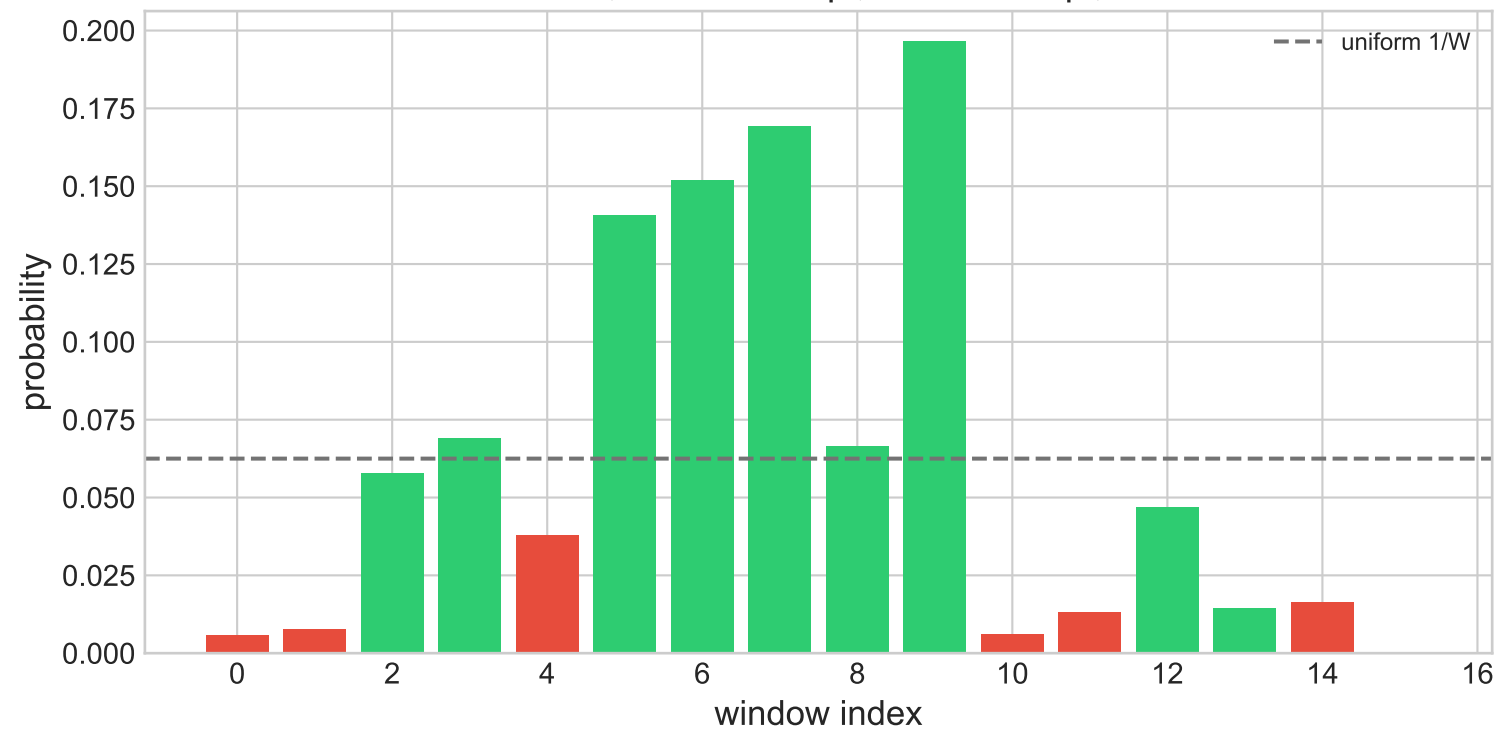
Optimal distribution - 08_2d_medium_clustered_obstacles P=0.9127 , \theta=0.964\pi , \beta=0.241\pi , r=36
