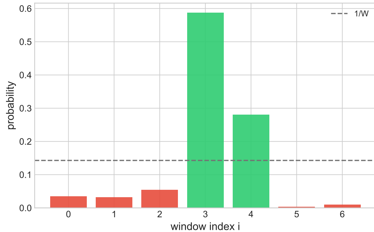
Distribution, P=0.8673
