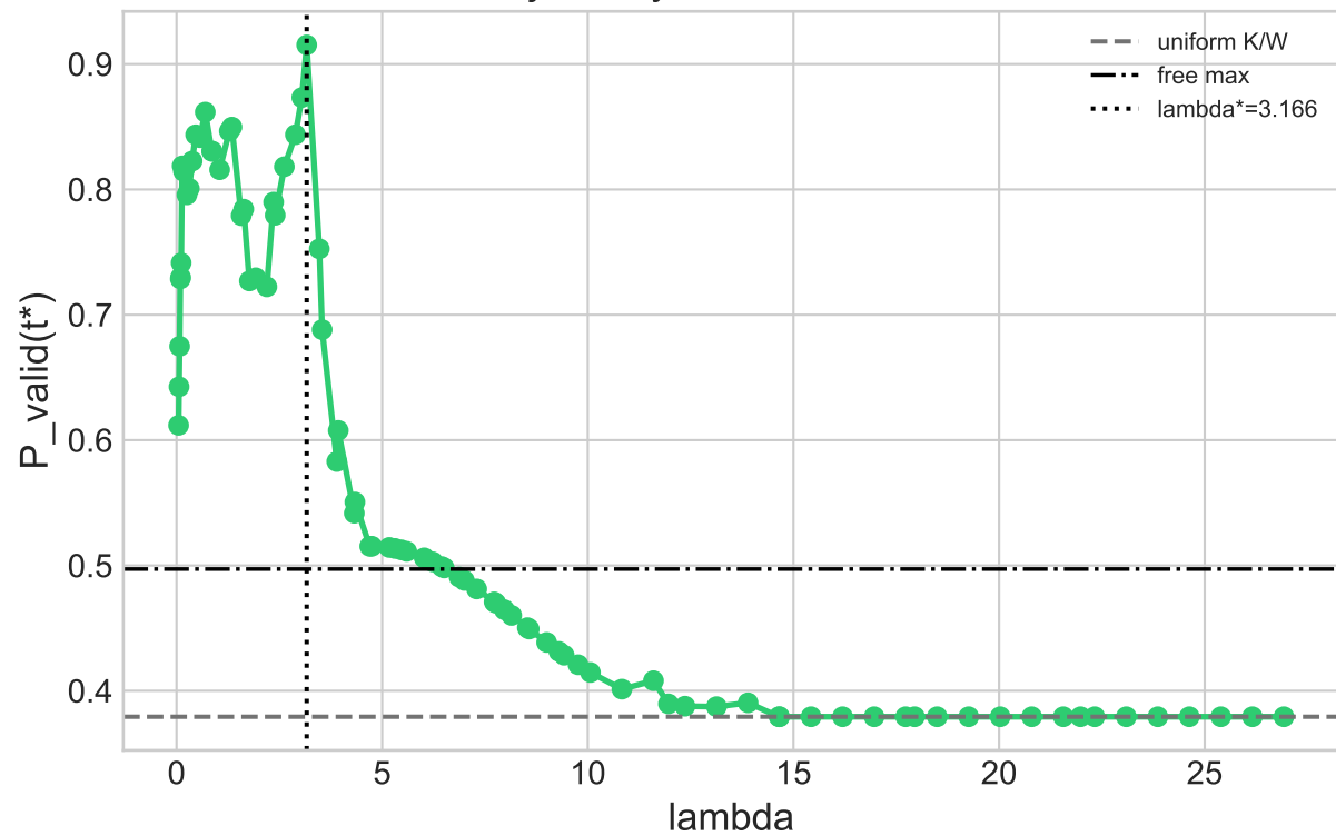
Distribution, P=0.9153
