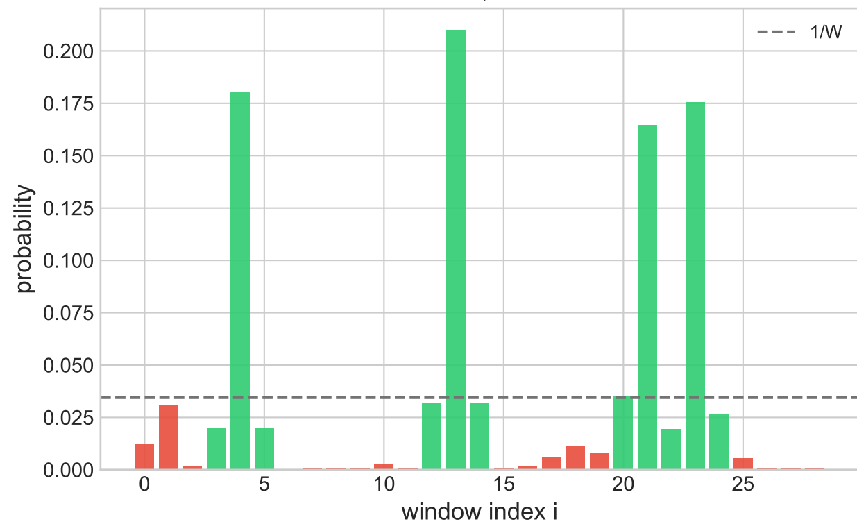
Distribution, P=0.9153
