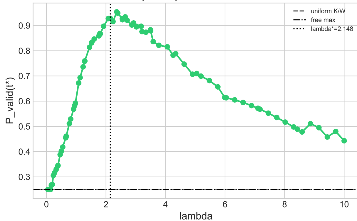
Distribution, P=0.9282
