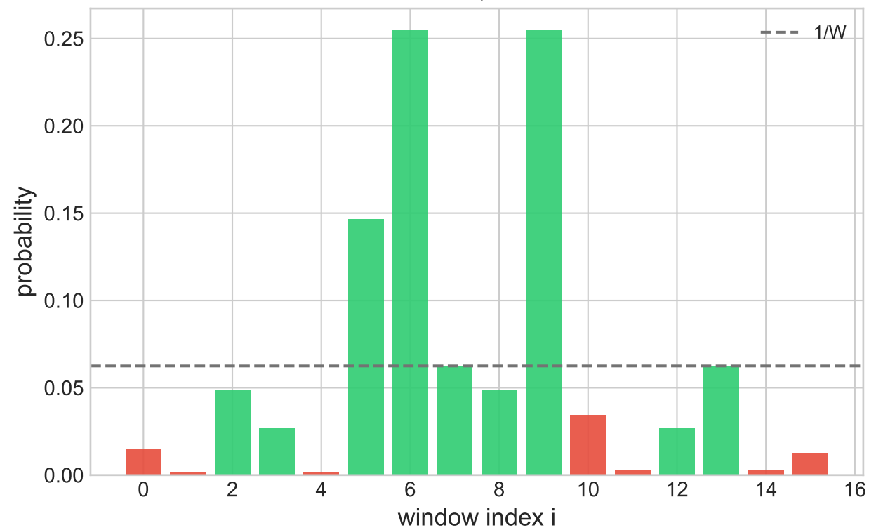
Distribution, P=0.9305
