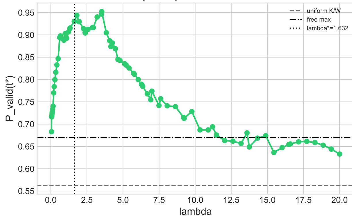
Distribution, P=0.9305
