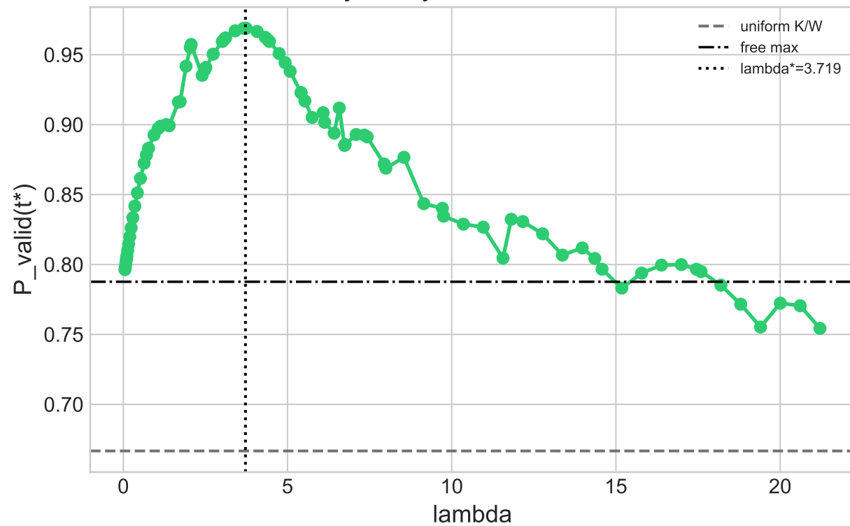
Distribution, P=0.9689
