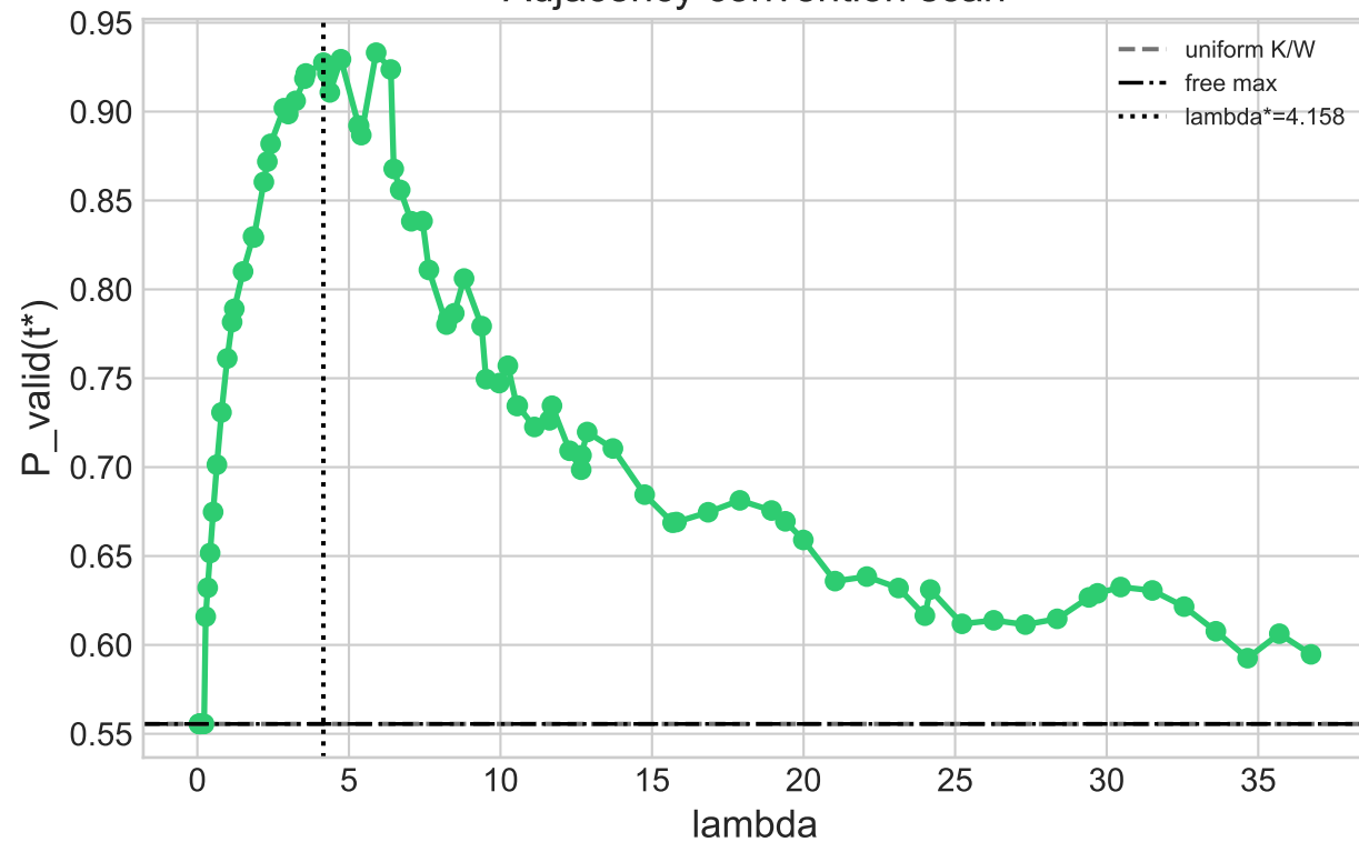
Distribution, P=0.9276
