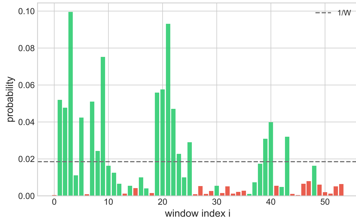
Distribution, P=0.9276
