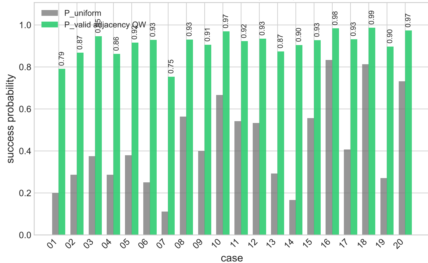
Uniform baseline vs adjacency QW
