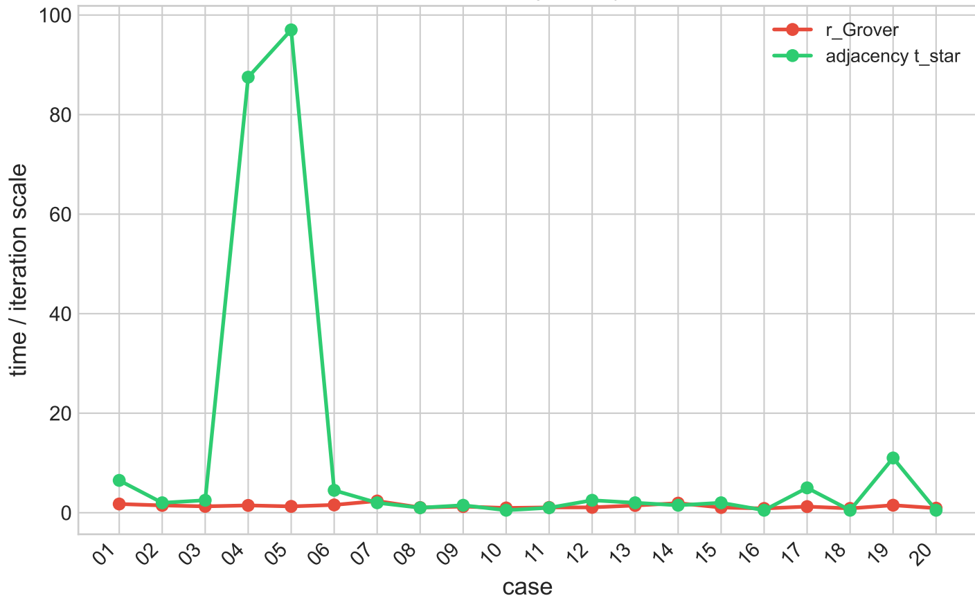
Grover scale vs adjacency QW time
