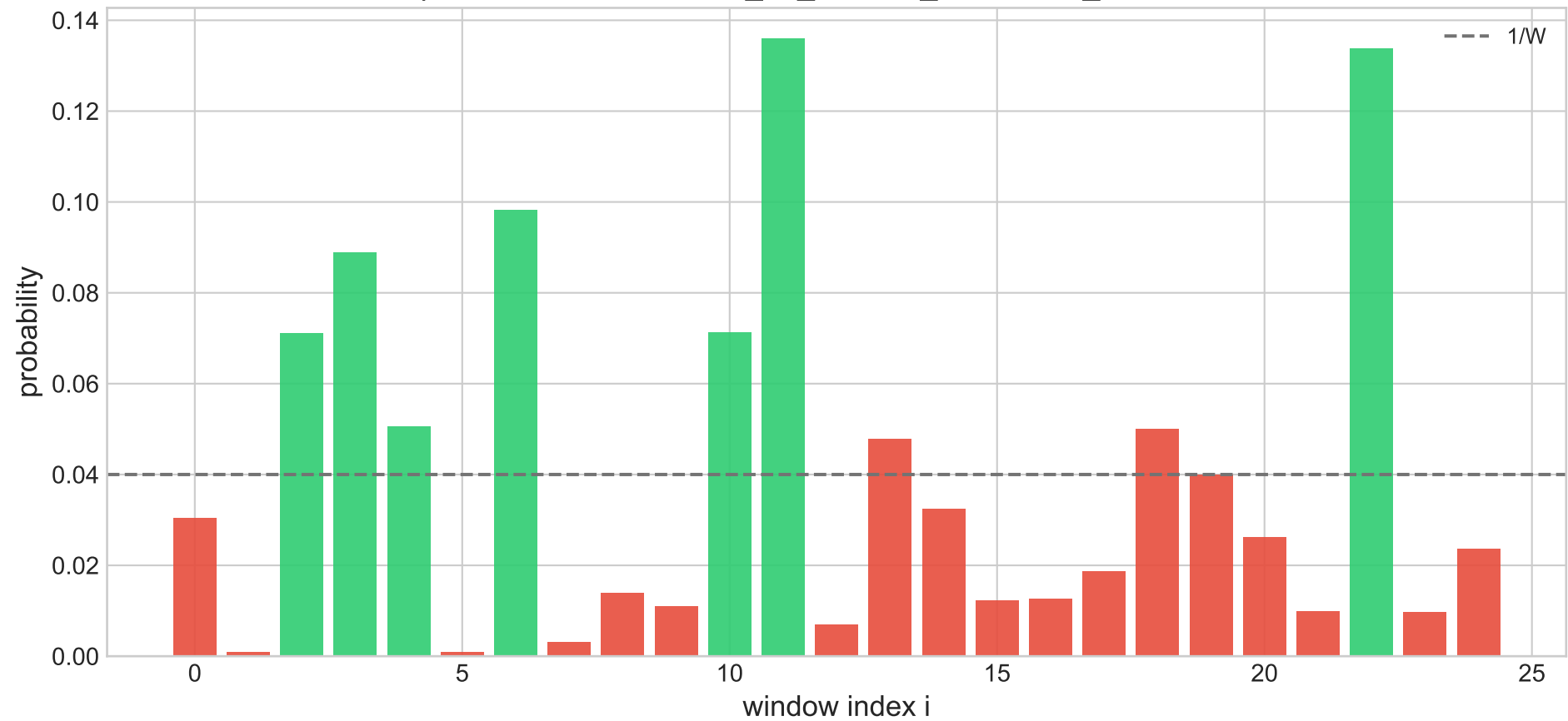
Optimal distribution — 13_2d_corridor_clusters, P_valid=0.6498
