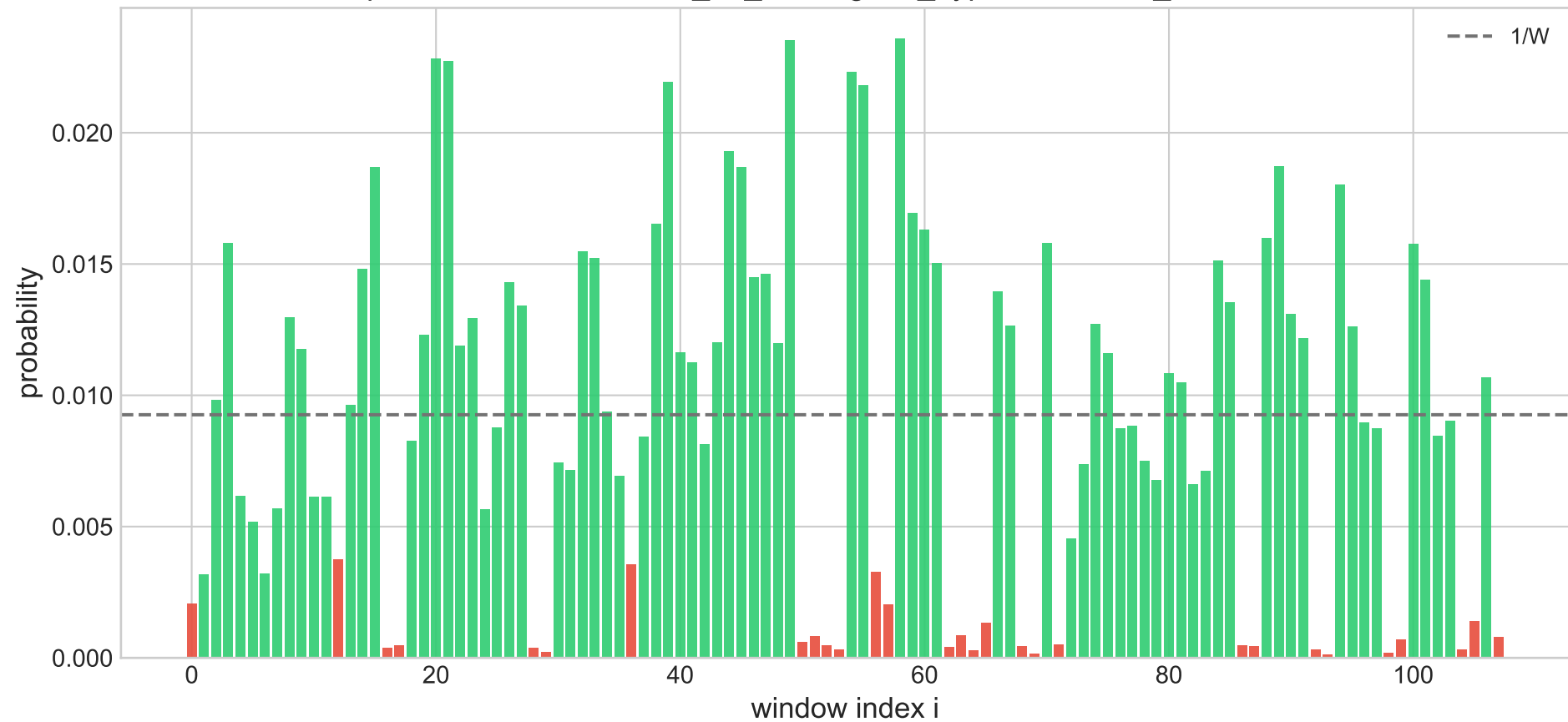
Optimal distribution — 20_5d_rectangular_hyperwindow, P_valid=0.9729
