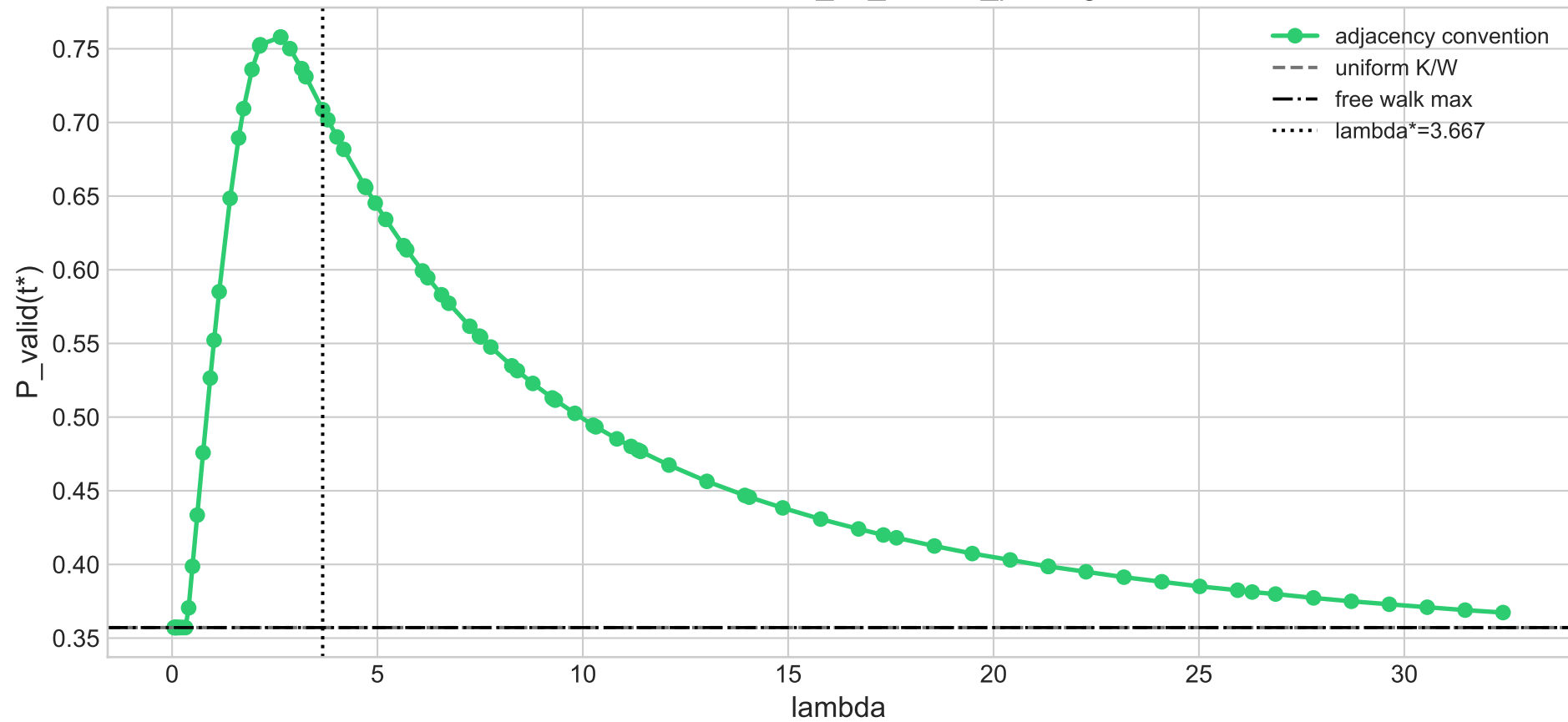
Lambda scan — 16_2d_narrow_passages
