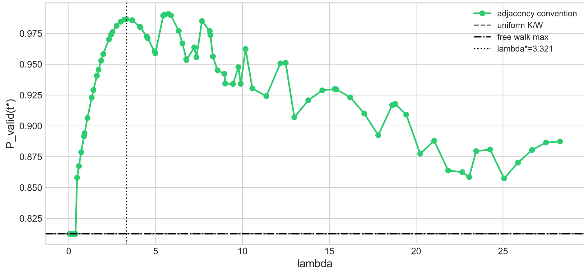
Lambda scan — 18_5d_tiny_hypercube_clusters
