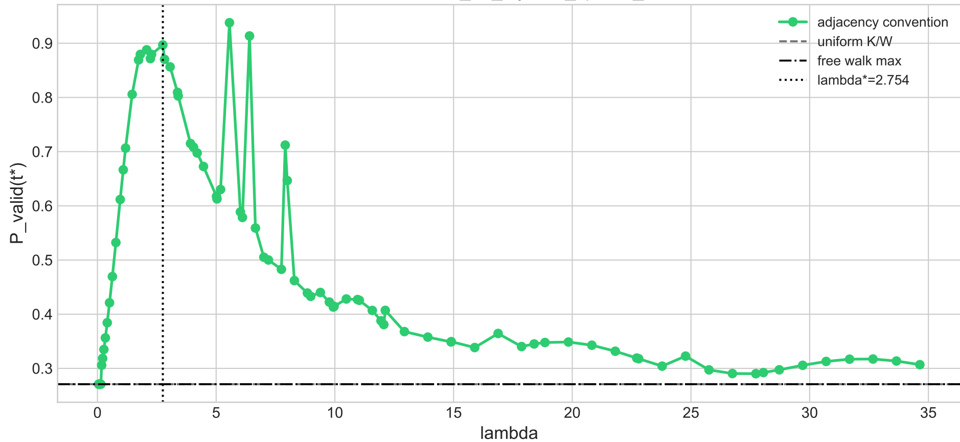
Lambda scan — 19_5d_layered_sparse_obstacles
