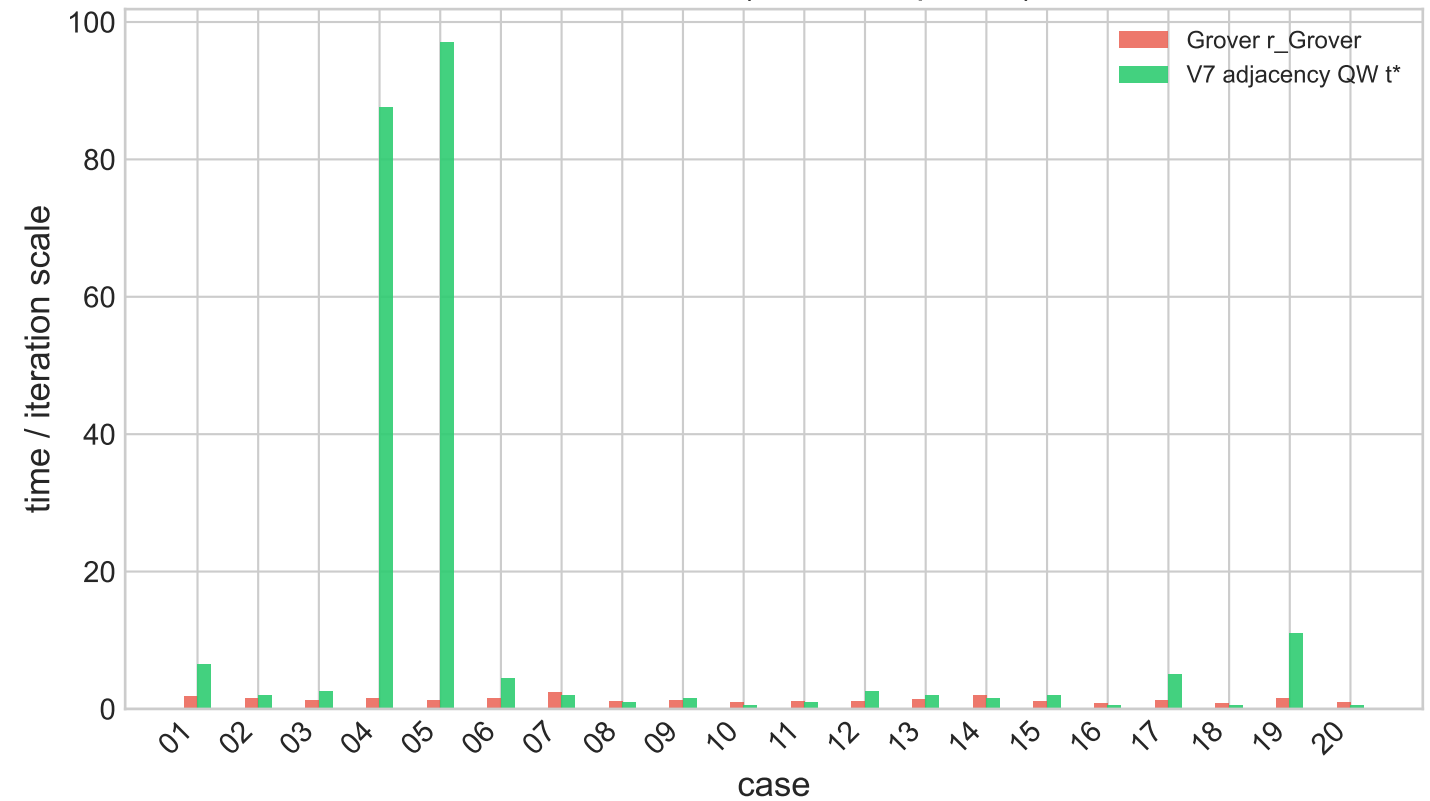
Time face-off (Grover cap OFF)
