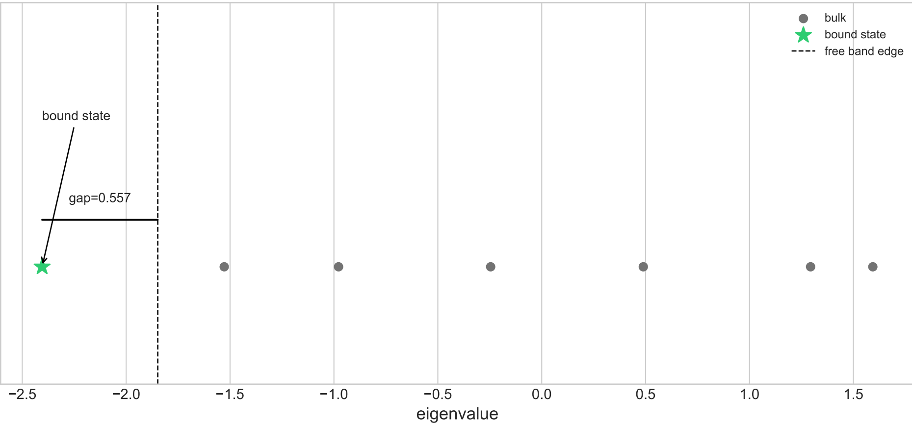
Eigenvalue spectrum — 02_1d_main_reference
