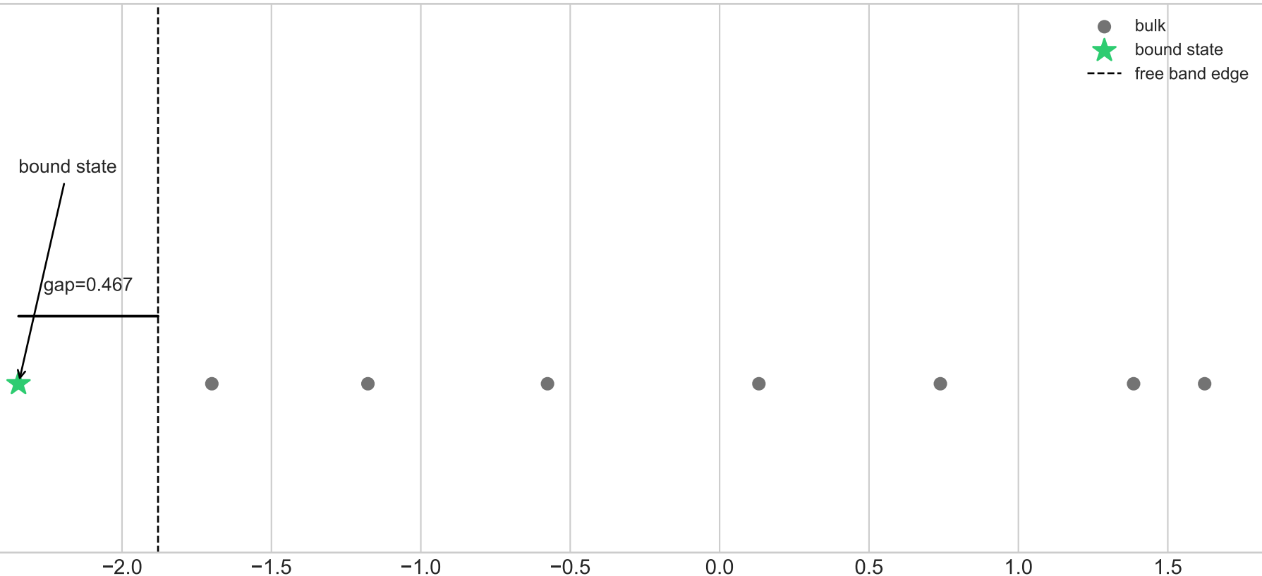
Eigenvalue spectrum — 03_1d_two_free_regions
