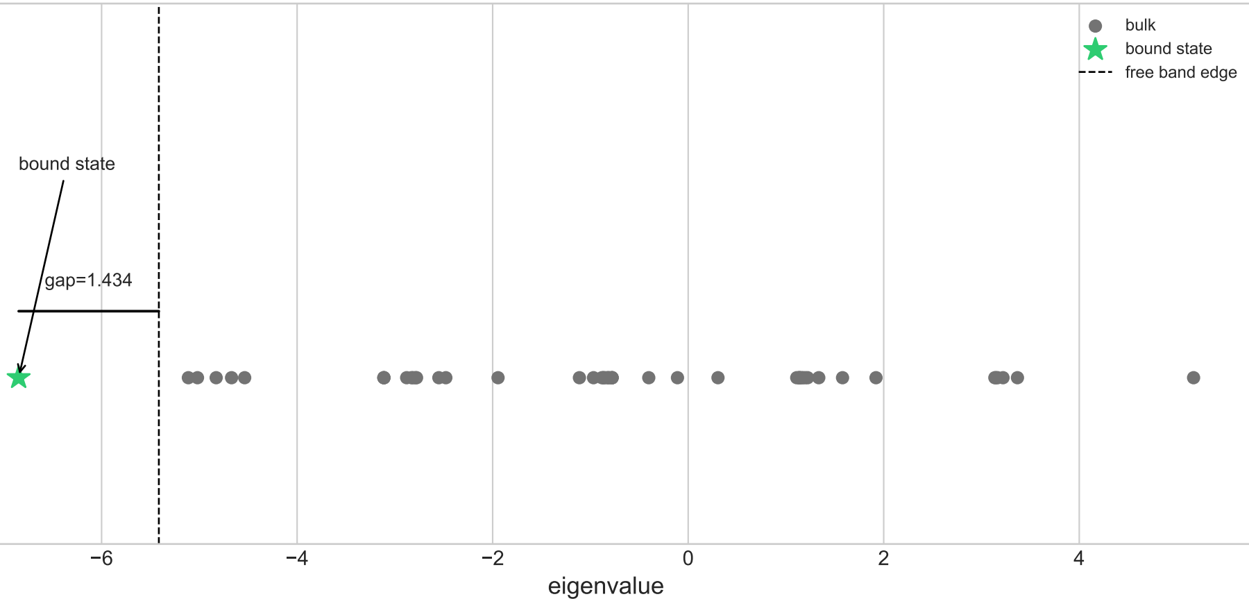
Eigenvalue spectrum — 19_5d_layered_sparse_obstacles
