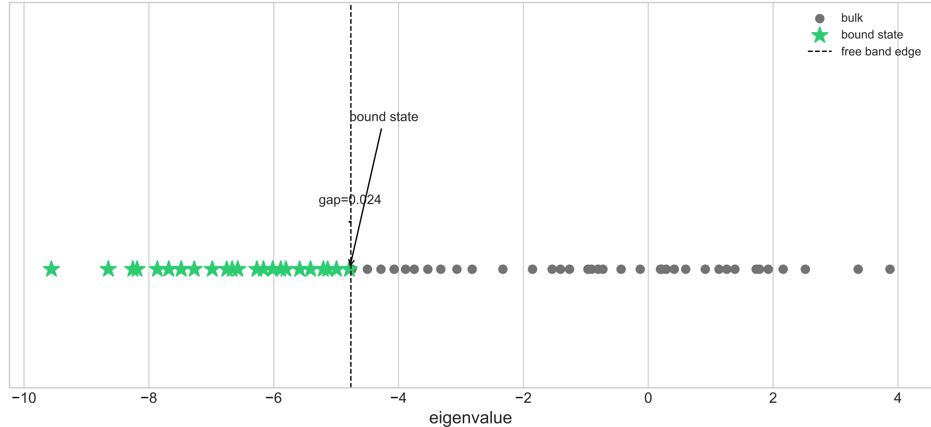
Eigenvalue spectrum — 20_3d_layered_obstacle_bands
