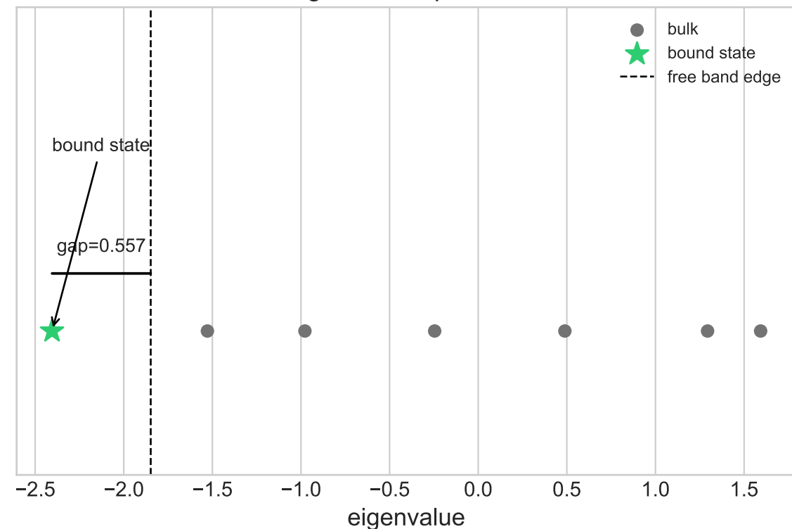
Lambda scan
