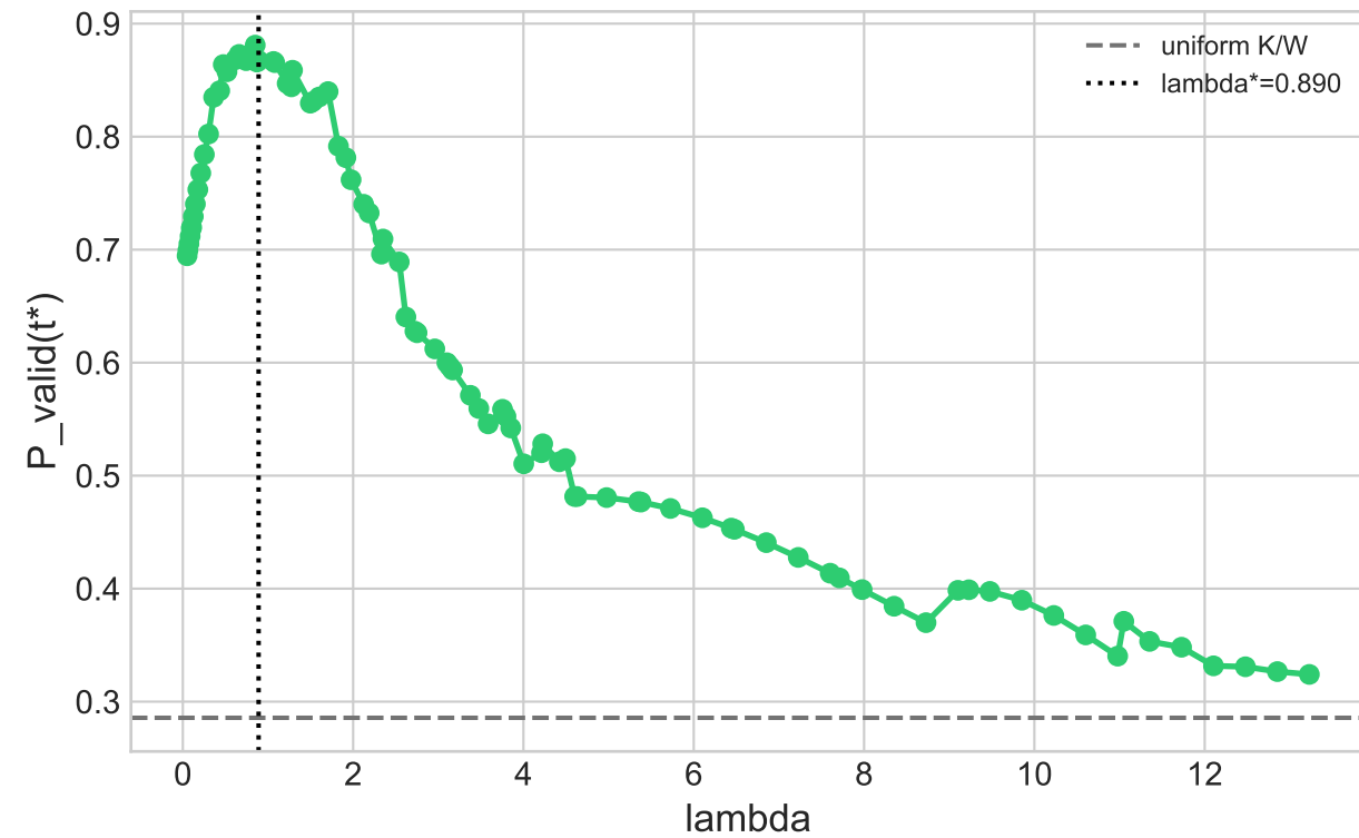
Lambda scan
