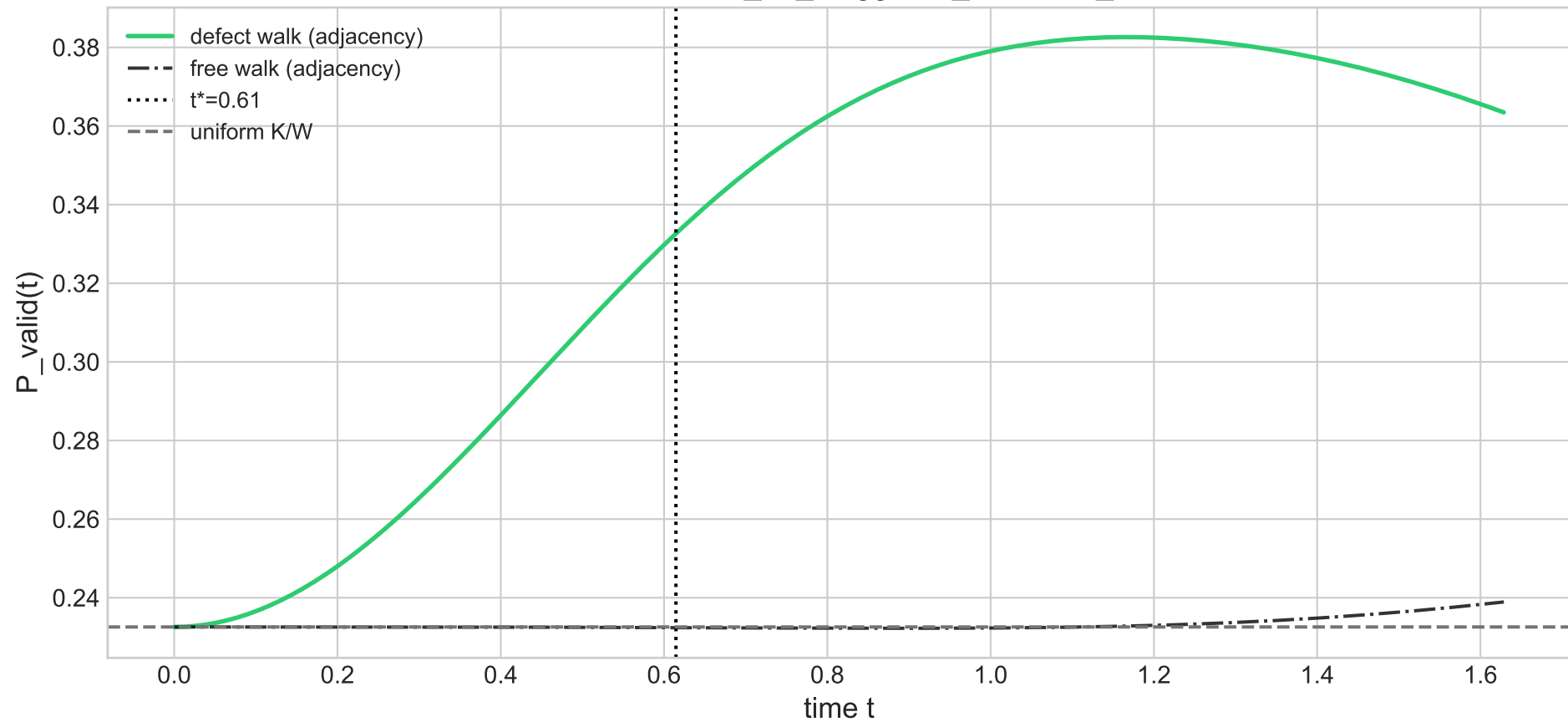
Time evolution — 12_1d_staggered_clustered_barriers
