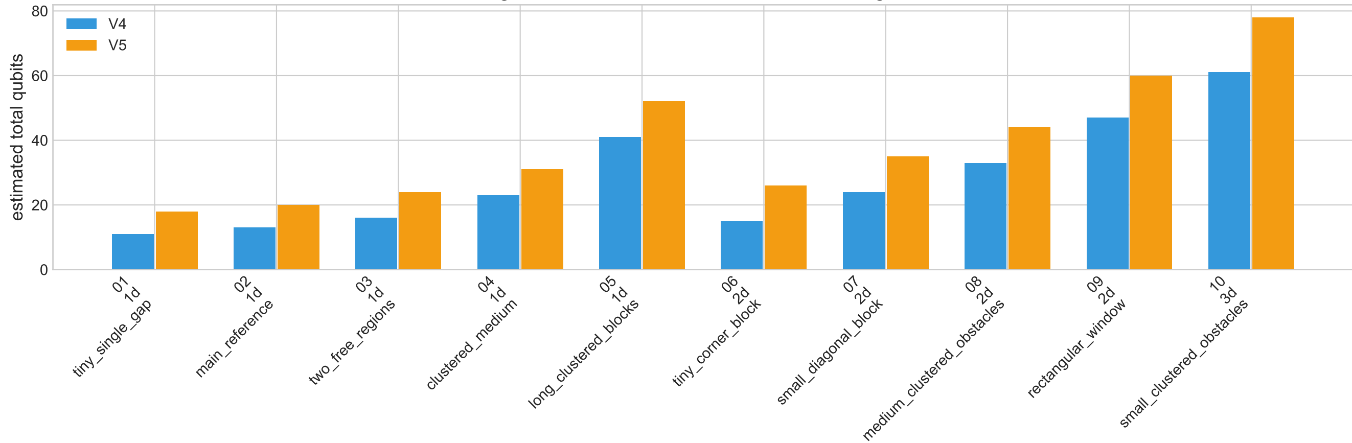
Register-size cost of V5 extra m2 and ancilla registers
