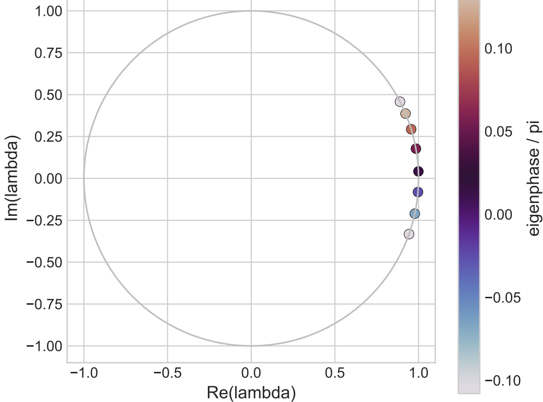
One-layer spectrum - 03_1d_two_free_regions
