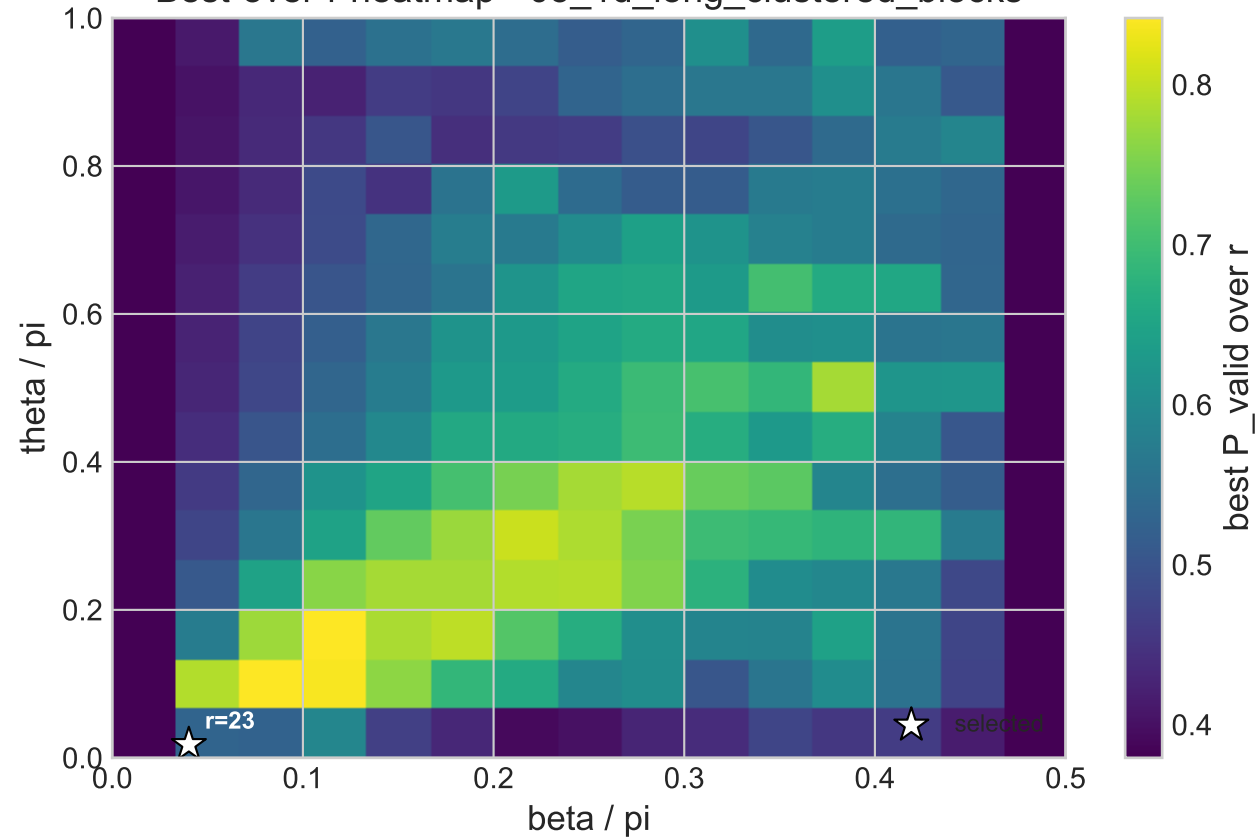
Best-over-r heatmap - 05_1d_long_clustered_blocks
