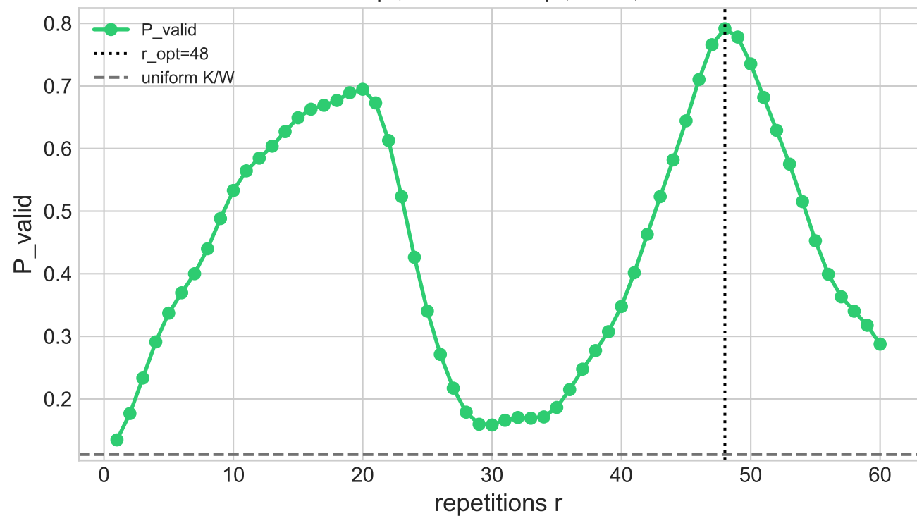
Oscillation - 07_2d_small_diagonal_block \theta=0.125\pi , \beta=0.054\pi , r=48 , P=0.7915
