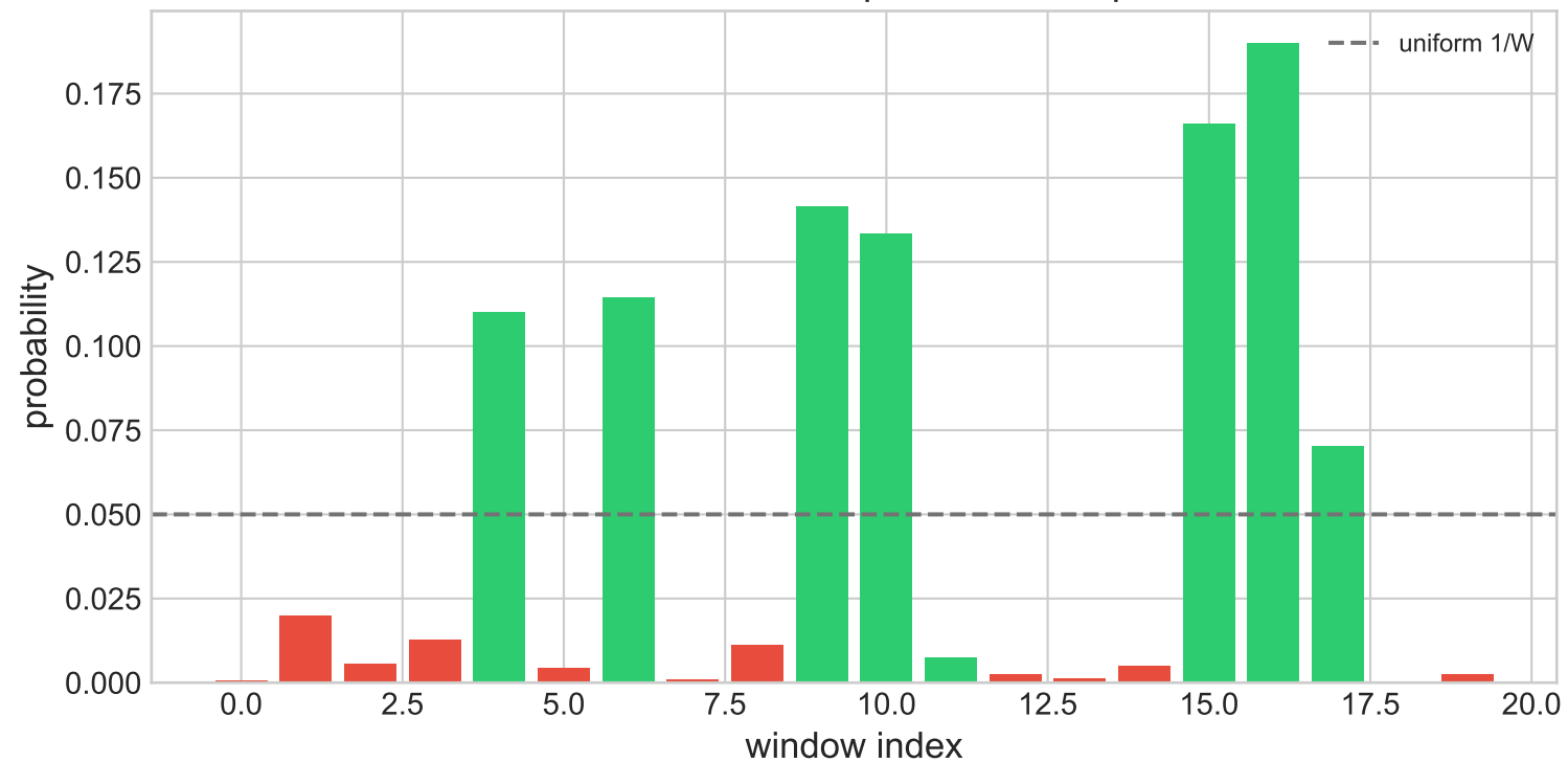
Optimal distribution - 09_2d_rectangular_window P=0.9332 , \theta=0.277\pi , \beta=0.250\pi , r=42
