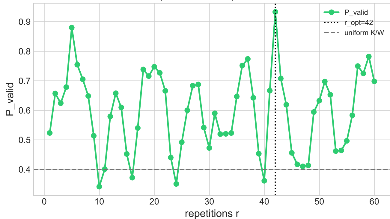
Oscillation - 09_2d_rectangular_window \theta=0.277\pi , \beta=0.250\pi , r=42 , P=0.9332
