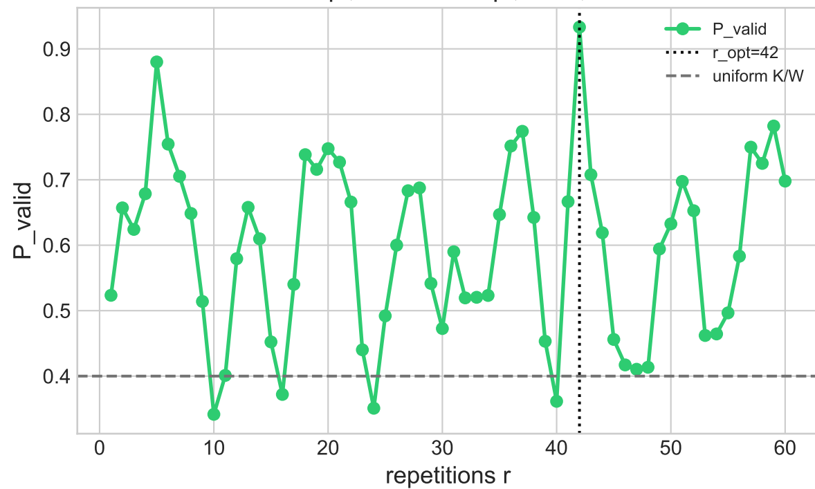
Oscillation - 09_2d_rectangular_window theta=0.277pi, beta=0.250pi, r=42, P=0.9332
