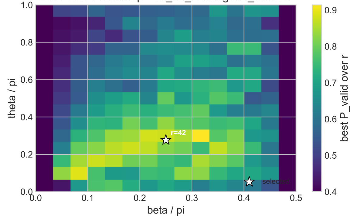
Optimal distribution - 09_2d_rectangular_window P=0.9332, theta=0.277pi, beta=0.250pi, r=42
