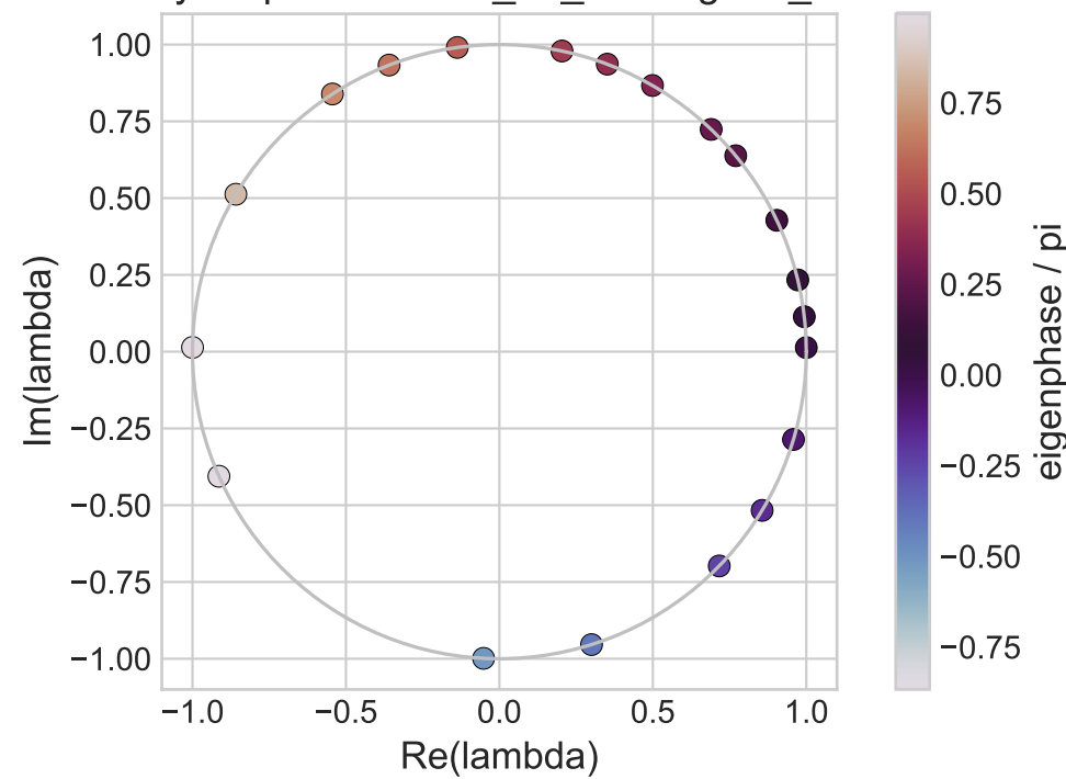
One-layer spectrum - 09_2d_rectangular_window
