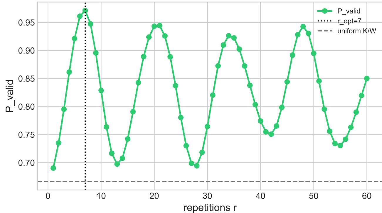
Oscillation - 10_3d_small_clustered_obstacles \theta=0.045\pi , \beta=0.027\pi , r=7 , \bar{P}=0.9711
