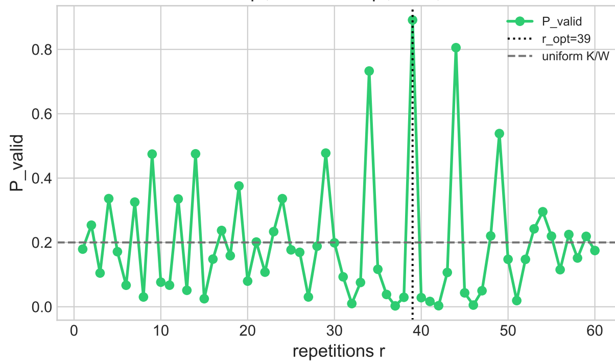
Oscillation - 01_1d_tiny_single_gap theta=0.679pi, beta=0.460pi, r=39, P=0.8913
