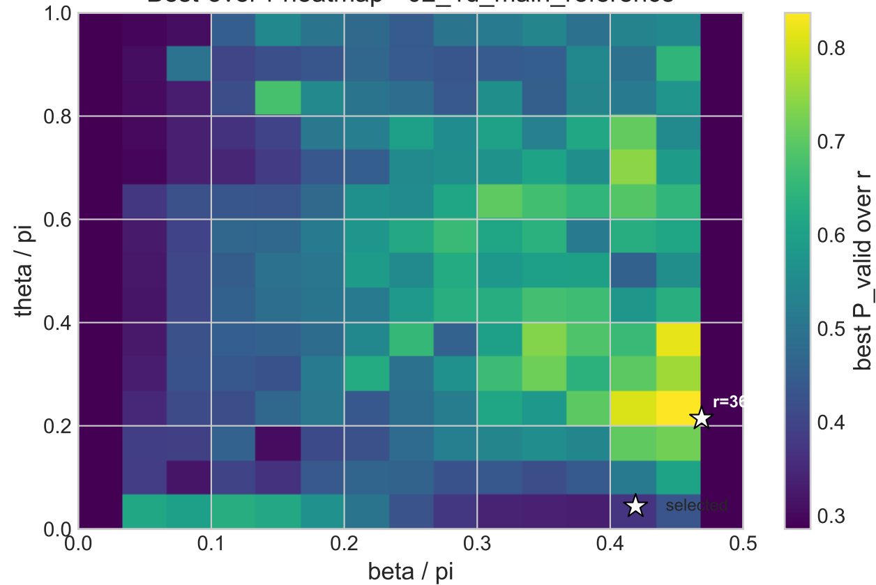
Best-over-r heatmap - 02_1d_main_reference
