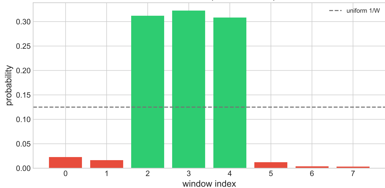
Optimal distribution - 03_1d_two_free_regions P=0.9427 , \theta=0.152\pi , \beta=0.344\pi , r=47
