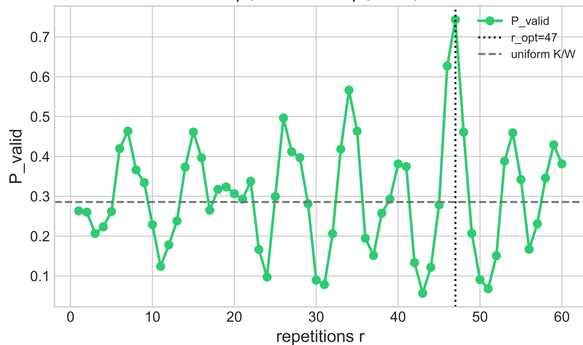
Oscillation - 04_1d_clustered_medium theta=0.223pi, beta=0.420pi, r=47, P=0.7433
