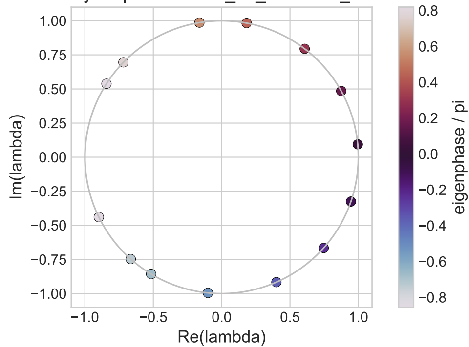
One-layer spectrum - 04_1d_clustered_medium
