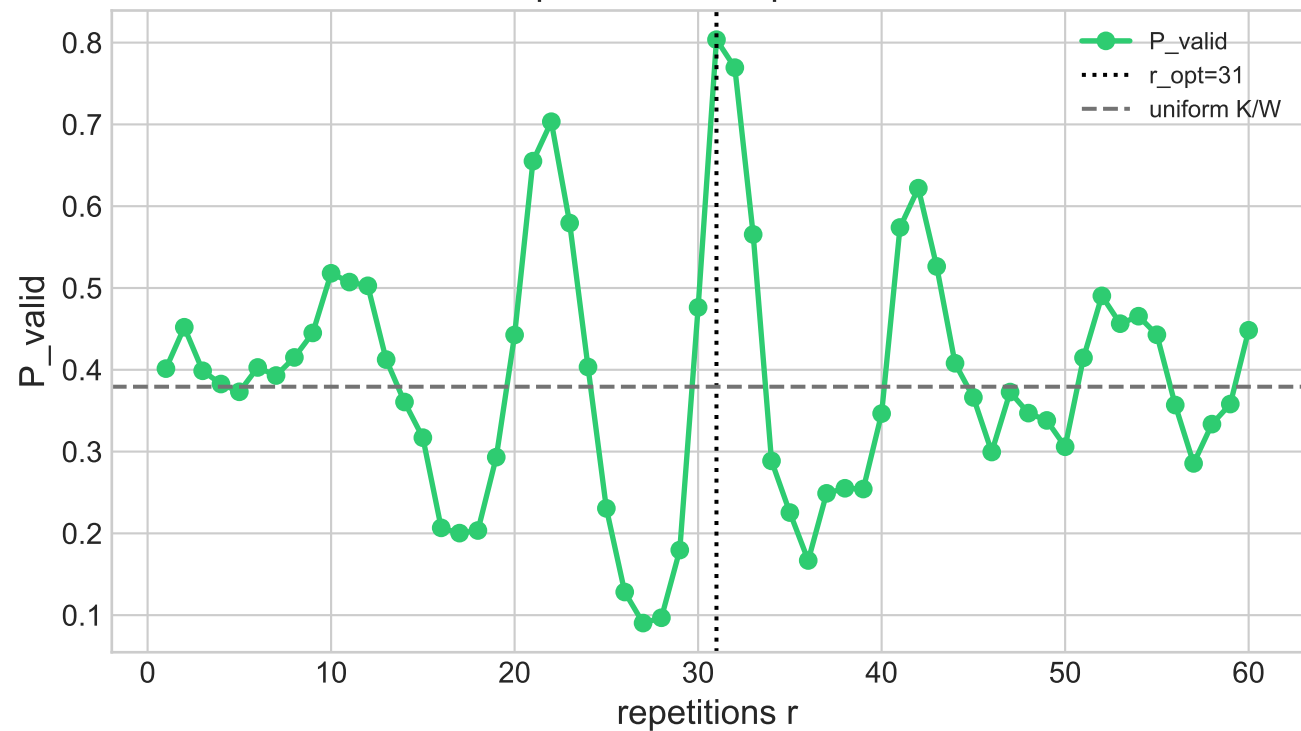
Oscillation - 05_1d_long_clustered_blocks \theta=0.295\pi , \beta=0.411\pi , r=31 , P=0.8036
