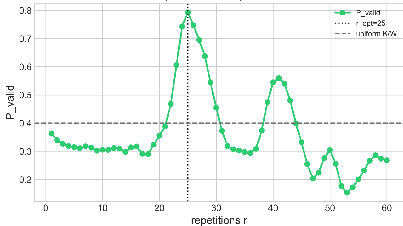
Oscillation - 09_2d_rectangular_window \theta=0.009\pi , \beta=0.138\pi , r=25 , P=0.7935
