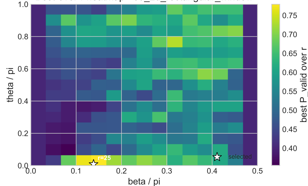
Optimal distribution - 09_2d_rectangular_window P=0.7935, theta=0.009pi, beta=0.138pi, r=25
