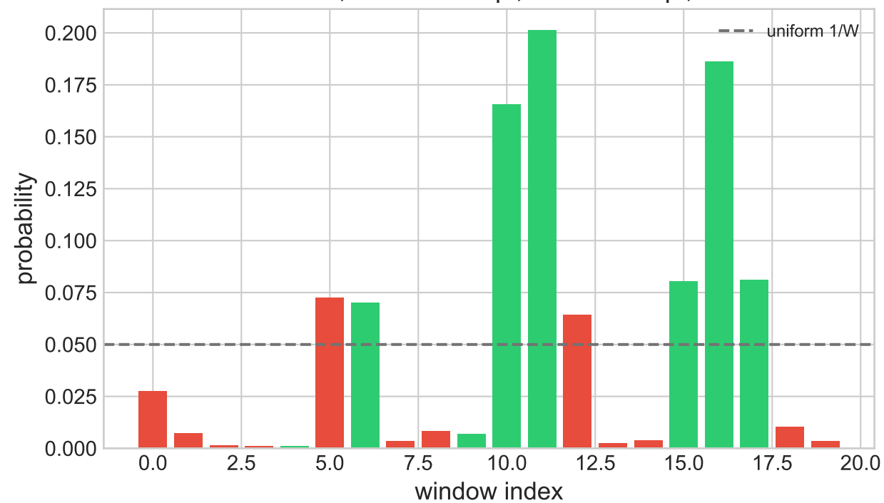
Optimal distribution - 09_2d_rectangular_window P=0.7935, theta=0.009pi, beta=0.138pi, r=25
