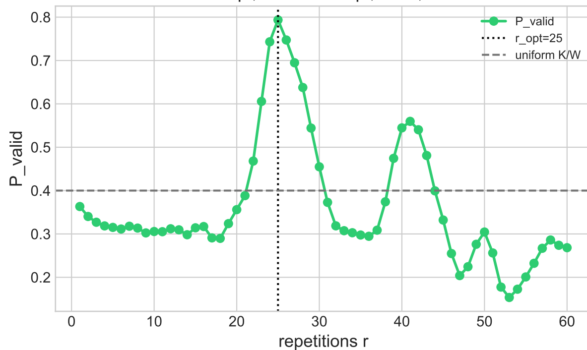
Oscillation - 09_2d_rectangular_window theta=0.009pi, beta=0.138pi, r=25, P=0.7935
