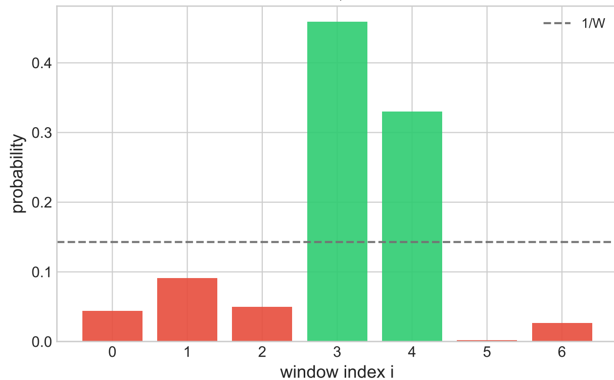
Distribution, P=0.7882
