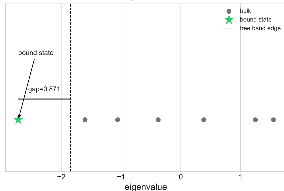
Spectrum
